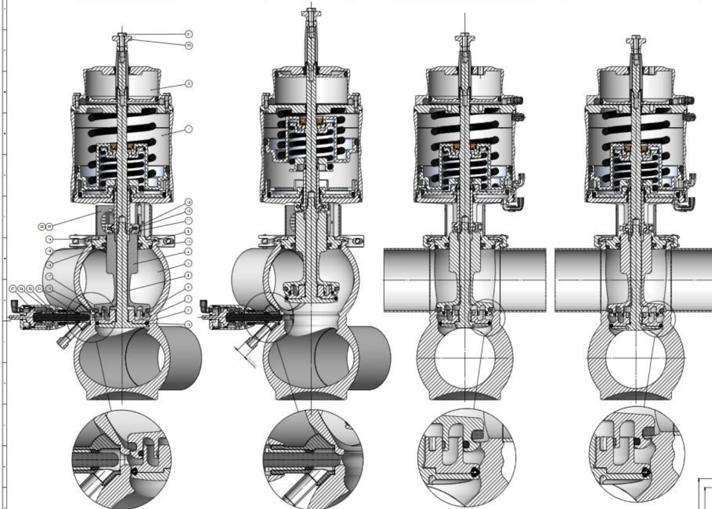
PROCESS VALVE CLOSED
